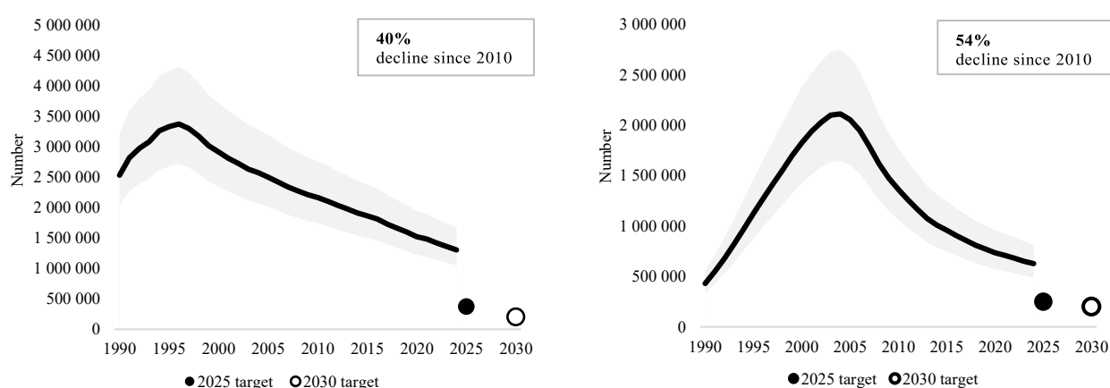
Figure I Numbers of new HIV infections and AIDS-related deaths, global, 1990–2024, and 2025 and 2030 targets New HIV infections AIDS-related deaths
